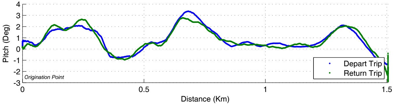
Vehicle Pitch Profile - Old Ridge Road, Archbald, PA.
