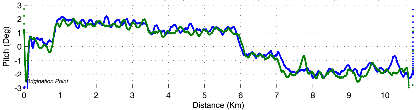
Vehicle Pitch Profile - Interstate Highway Route-81:Exit 217 (Harford) to Exit 223 (New Milford), PA.
