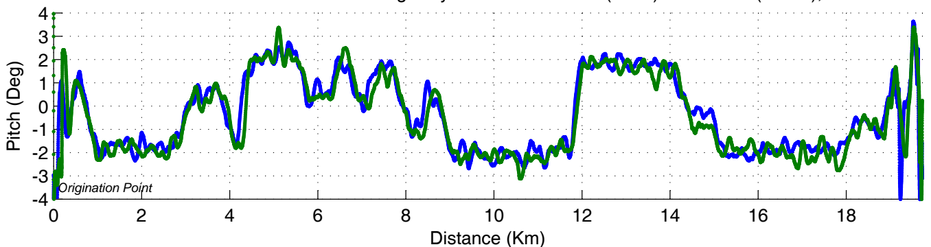
Vehicle Pitch Profile - Interstate Highway Route-81:Exit 199 (Scott) to Exit 211 (Lenox), PA.
